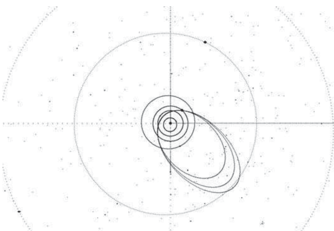
Figure 5. Triangulated orbits for the meteor captured in Figure 3.
