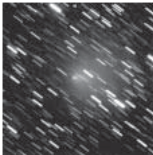
Comet 2P/Encke recorded by Martin Moberley at 2003 November 16.780 UT. 11×20s exps., C14 at f/7.7, ST9XE CCD.
