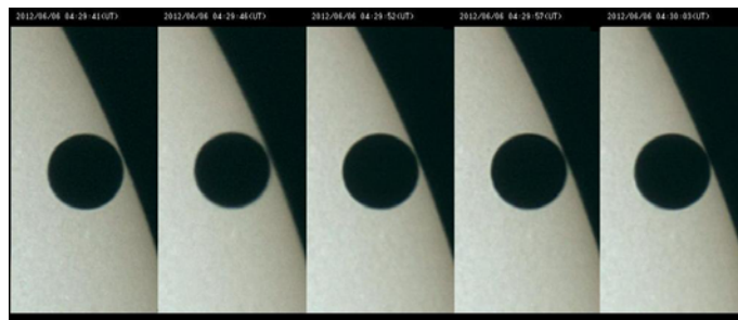
Figure 12. Third contact imaged from Japan with 380mm refl. stopped to 180mm and DFK51AU02 camera. T. Ikemura. From left to right, the results of 12 fps 3 second avi movies at 04:29:41UT, 04:29:46UT, 04:29:52UT, 04:29:57UT and 04:30:03UT. Note the complete absence of any Black Drop.
