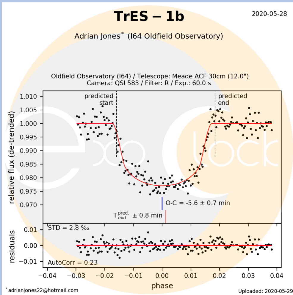
Transit light-curve of TrES-1b
