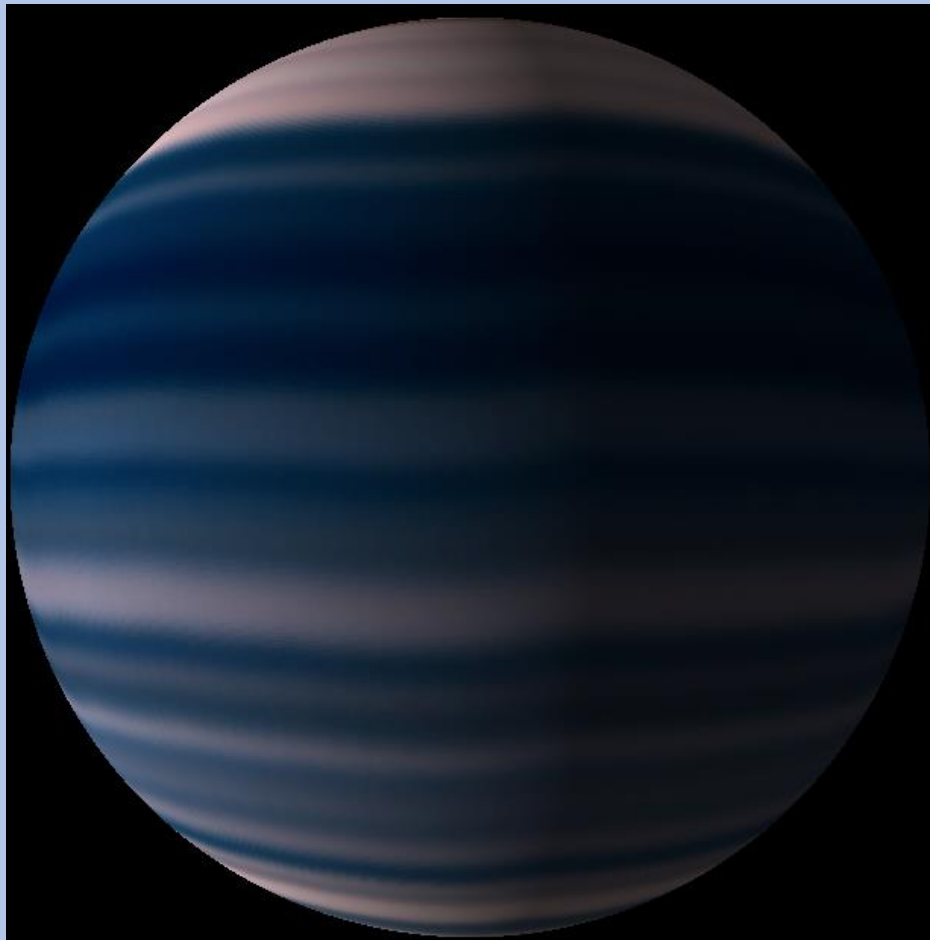
Artists impression of TrES-1b
