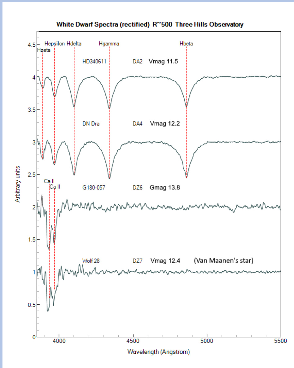
White Dwarf Spectra
