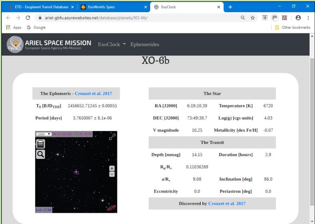
Figure A2.1 Star and transit data
