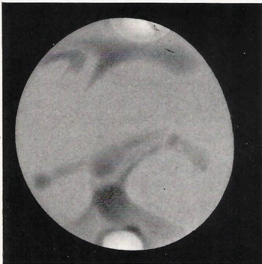
FIG. 3.—T. E. R. PHILLIPS. 12\frac{1}{4} -in. Spec. 1916, March 31. \omega = 40^\circ , \phi = + 14^\circ.9 .
