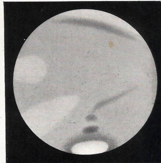
FIG. 6.—T. E. R. PHILLIPS. 12\frac{1}{4} -in. Spec. 1916, February 8. \omega = 134^\circ , \phi = + 16^\circ.3 .
