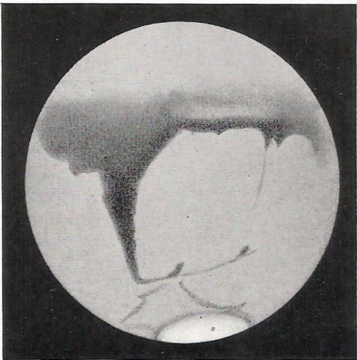
FIG. 4.—W. F. A. ELLISON. 18-in. Spec. 1916, January 22. \omega = 304^\circ , \phi = + 18^\circ.0 .
