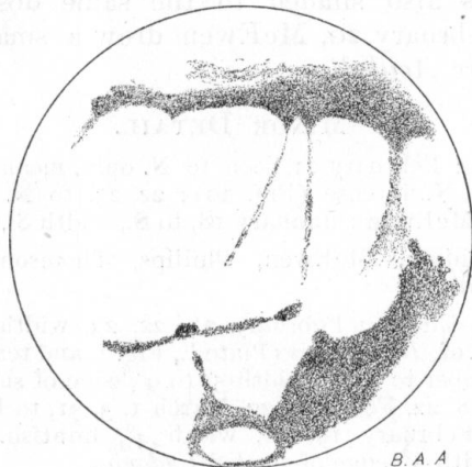
FIG. 10.— Sinus Sabæus and Mare Acidalium , 1916, February 21, \omega = 351^\circ . (Ellison.)
