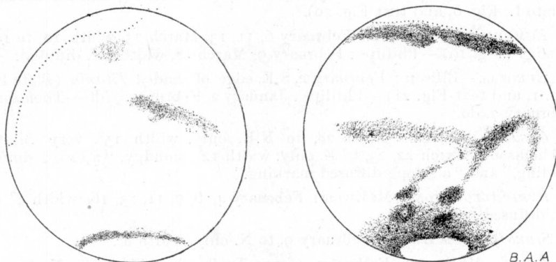
FIG. 19.—March 23, \omega = 124^\circ . (McEwen.)
