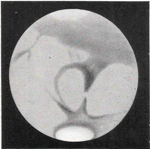
FIG. 3.—H. THOMSON. 12 \frac{1}{4} -in. Spec. 1916, March 3. \omega = 265^\circ , \phi = + 14^\circ.4 .
