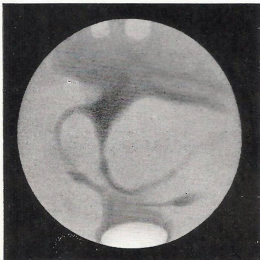
FIG. 5.—H. THOMSON. 12 \frac{1}{4} -in. Spec. 1916, March 3. \omega = 297^\circ , \phi = + 14^\circ.4 .
