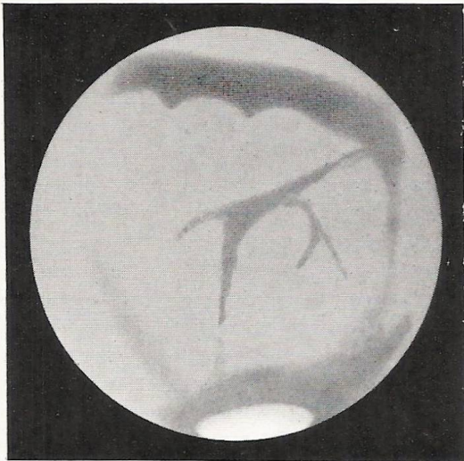
FIG. 1.—W. F. A. ELLISON. 18-in. Spec. 1916, February 2. \omega = 193^\circ , \phi = + 16^\circ.9 .
