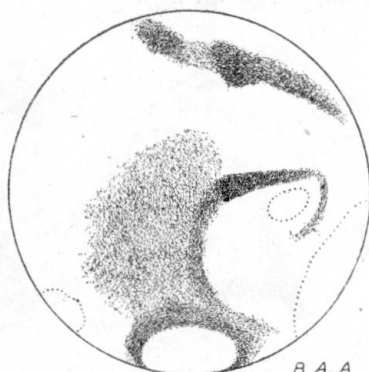
FIG. 22.—February 2, \omega = 186^{\circ} . (Thomson.)
