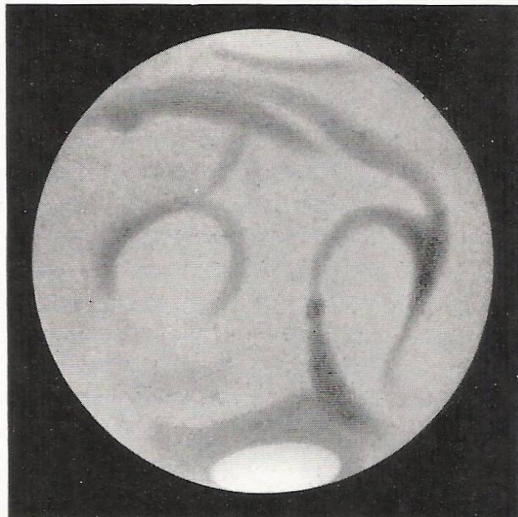
FIG. 2.—T. E. R. PHILLIPS. 12 \frac{1}{4} -in. Spec. 1916, February 6. \omega = 240^\circ , \phi = + 16^\circ.6 .
