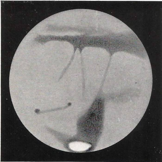
FIG. 1.—W. F. A. ELLISON. 18-in. Spec. 1916, February 21. \omega = 13^\circ , \phi = + 15^\circ.0 .
