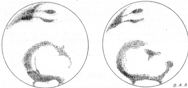
FIG. 17.—February 20, \omega = 74^\circ .
