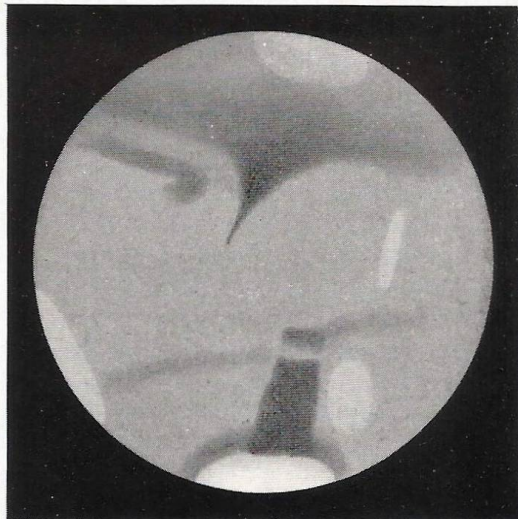
FIG. 2.—H. THOMSON. 12\frac{1}{4} -in. Spec. 1916, February 19. \omega = 16^\circ , \phi = + 15^\circ.2 .
