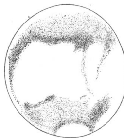
FIG. 9.—March 31, \omega = 351^\circ . (The Director.)
