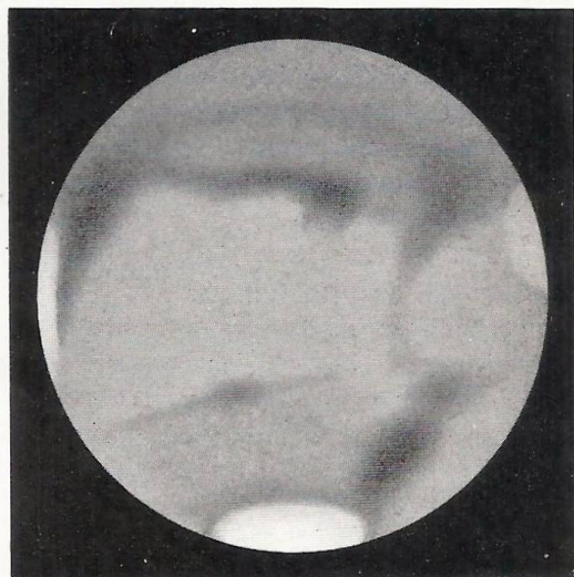
FIG. 6.—E. M. ANTONIADI. 8 \frac{1}{2} -in. Spec. 1916, February 20. \omega = 349^\circ , \phi = + 15^\circ.2 .
