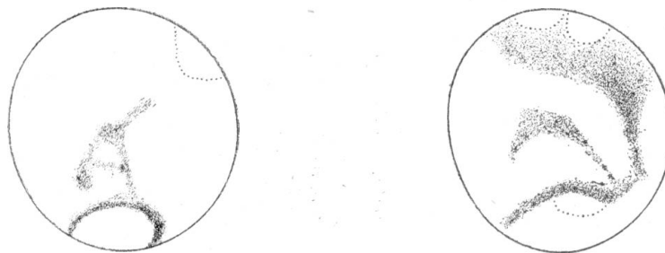
FIG. 26.—December 26, \omega = 215^\circ .
