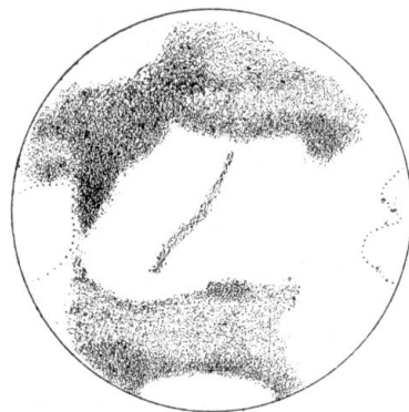
FIG. 32.—February 24, \omega = 322^\circ .
