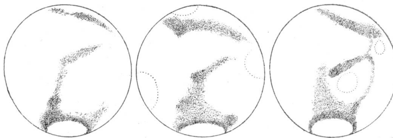
FIG. 23.—January 2, \omega = 191^\circ . (Phillips.)
