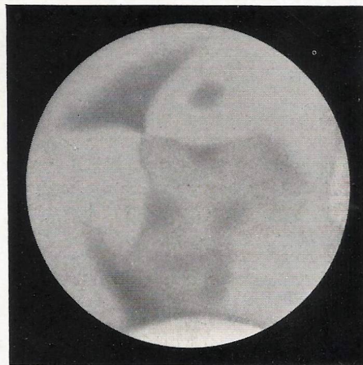
FIG. 4.—H. MCEWEN. 5-in. O.G. 1916, February 16. \omega = 79^\circ , \phi = + 15^\circ.5 .
