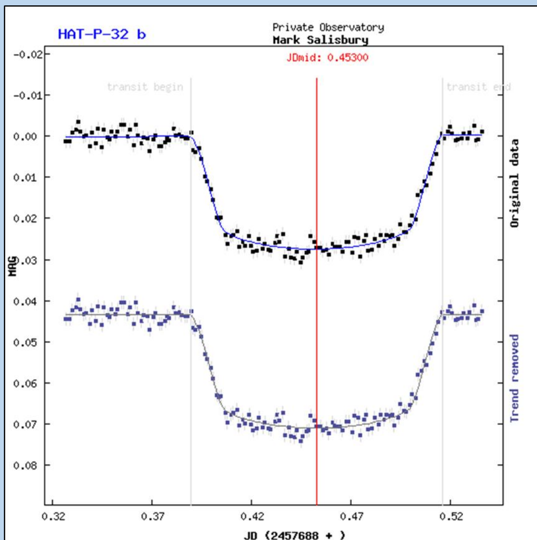
Figure 1. Transit light curve of HAT-P-32 b obtained by Mark Salisbury using a 0.4m f6.8 telescope plus SBIG ST10XME CCD camera
