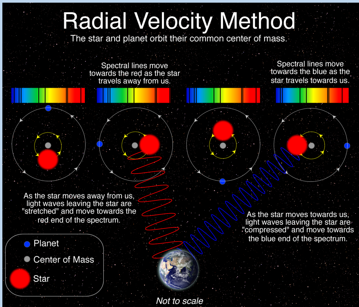
Figure 3. Detecting exoplanets by the radial velocity method.
