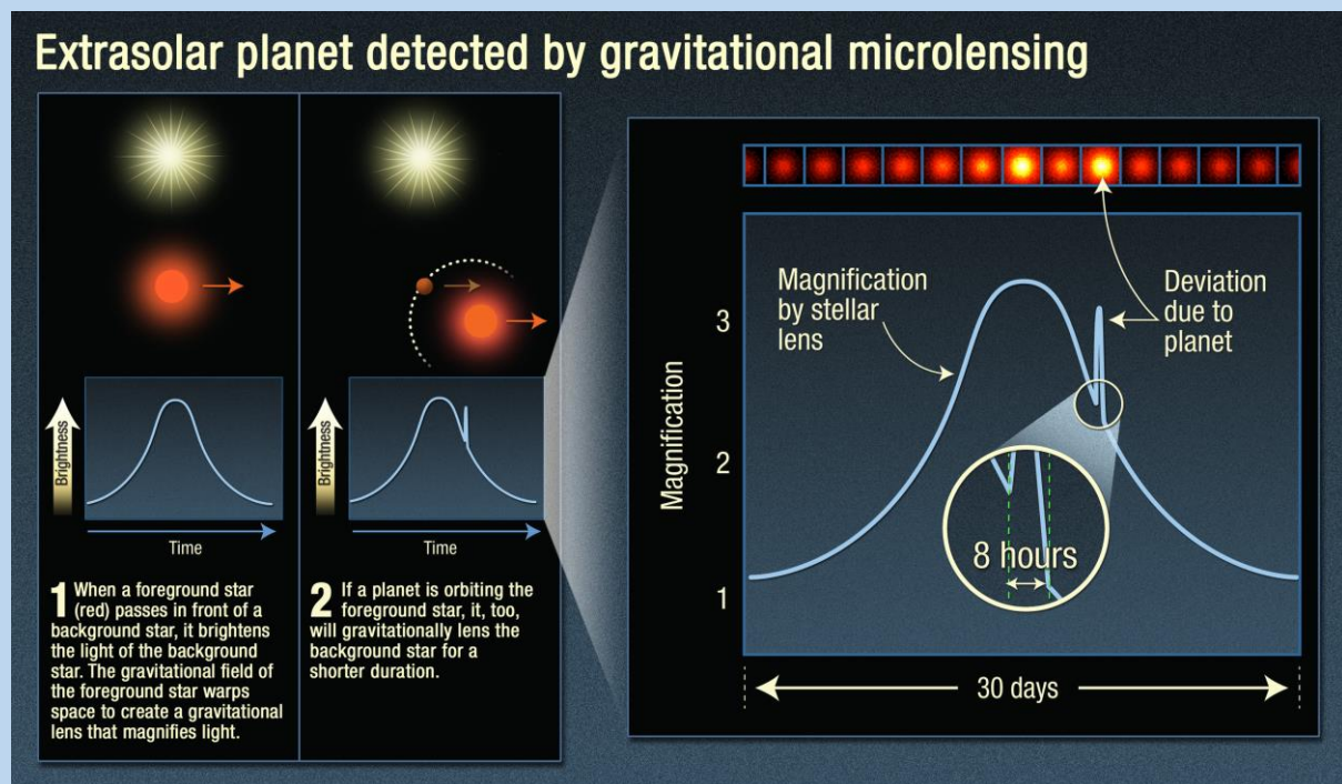
Figure 2. Gravitational microlensing
