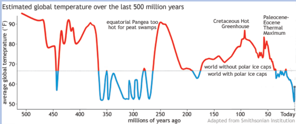
Earth's temperature
