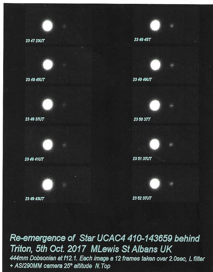
Figure 13. Occultation of the star UCAC4 410-143659 by Triton on 2017 Oct 5. Duration 144s. (M. Lewis)
