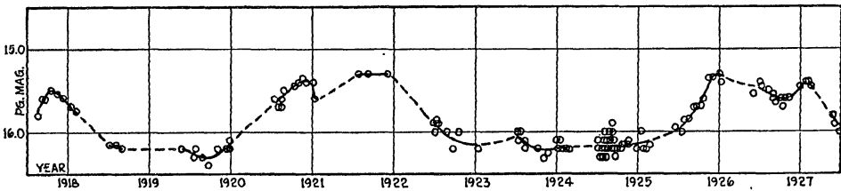
FIG. 4.—Light-curve of variable No. 19
