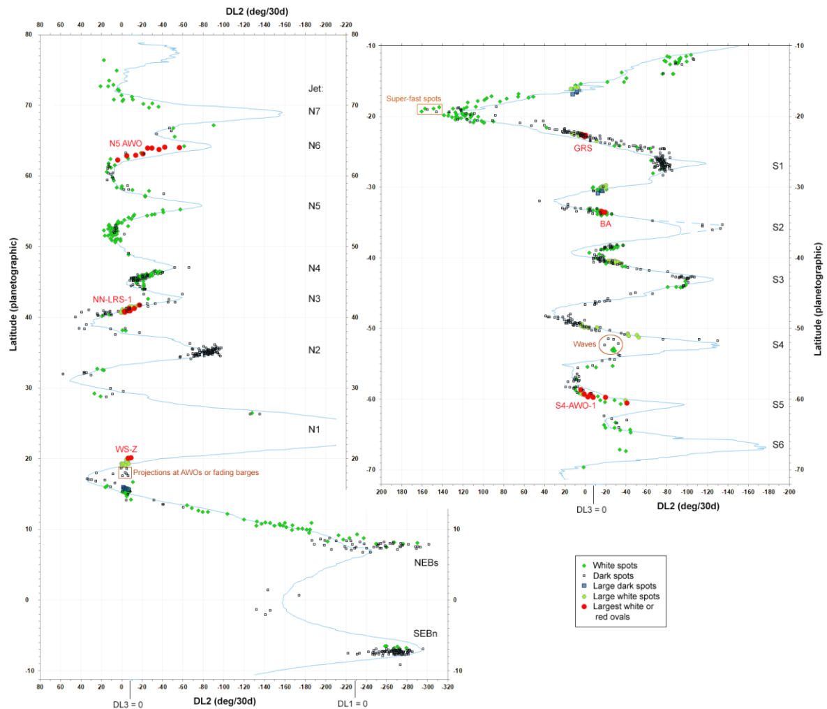
Figure 2. ZDP covering most of the planet, 2022/23, from JUPOS data (from Report 2022/23 no.10 ).
