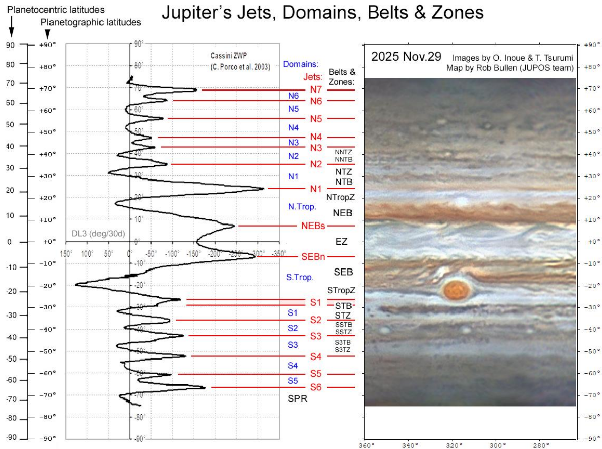
Figure 1: Definitions of Jupiter's jets, domains, belts & zones, by latitude.
